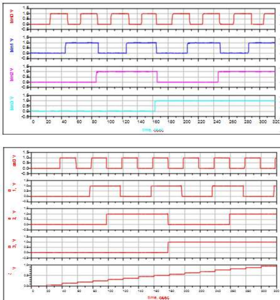
Fig 4 Simulation Results for Pipeline ADC
