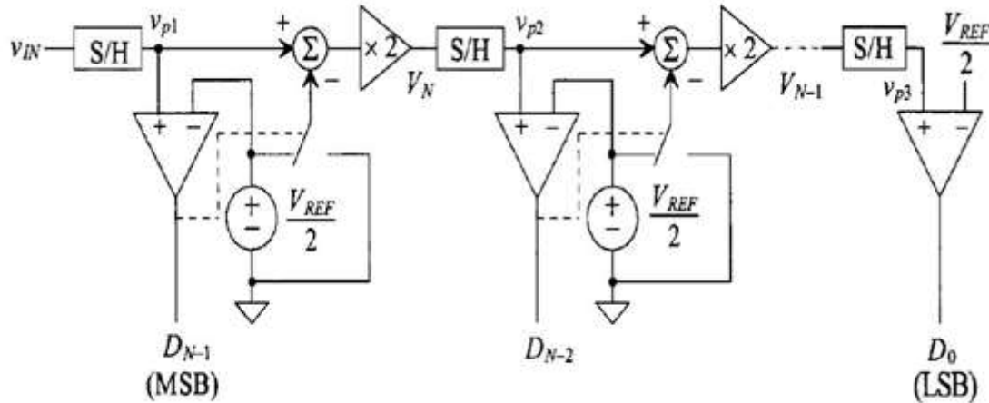
Fig 1 pipeline A/D converter
