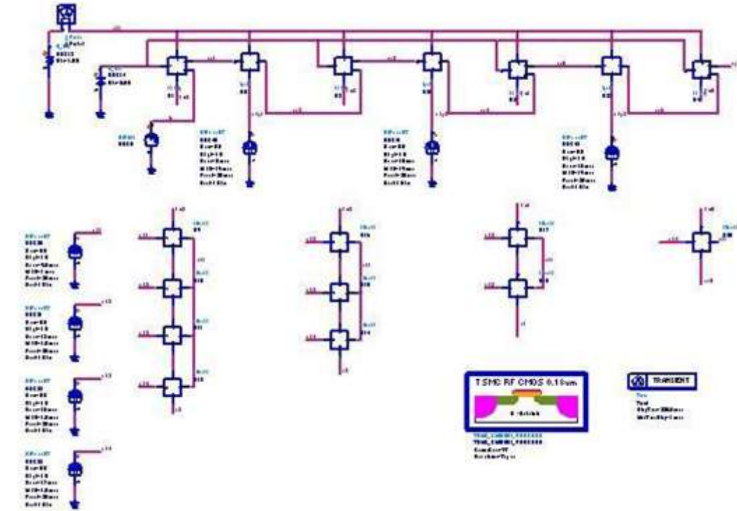
Fig 3 Pipeline Architecture
