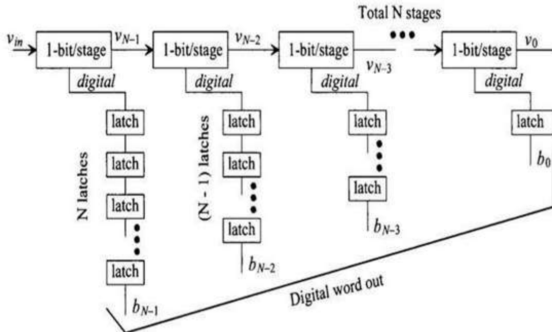
Fig 2. Pipeline ADC based on cyclic stages
